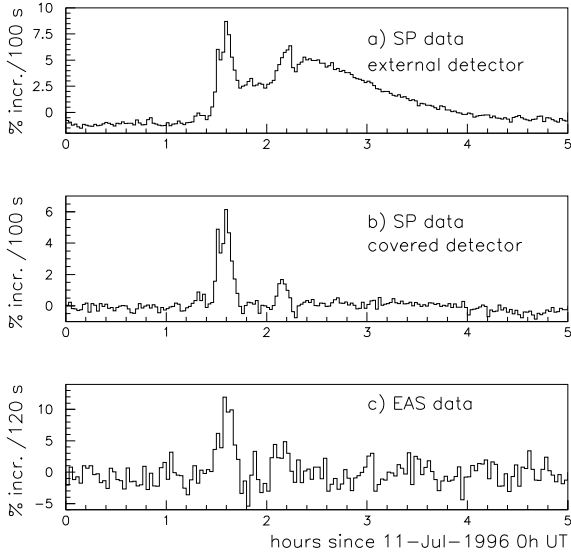
Fig. 1. EAS-TOP data during the July 11 event. Curve a : percent increase of the single particle counting rate of one “external” detector; curve b : single particle counting rate of one “covered” detector; curve c : extensive air shower rate.
