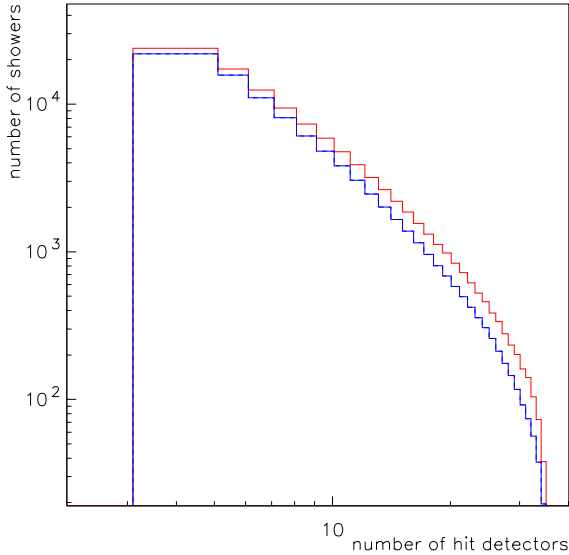
Fig. 3. Integral distribution of the number of hit detectors per shower during the EAS increase of July 11 1996 (red line) and in condition of unperturbed weather conditions (blue line).
