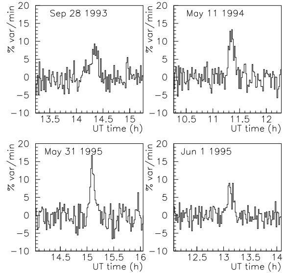
Fig. 2. Percent variation per minute of the showers counting rate during 2 hours around four EAS increase events.
