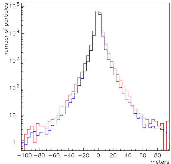
Fig. 5. Distance of the shower particles from the best fit plane of the shower front during the EAS increase of July 11 1996 (red line) and during normal conditions (blue line).
