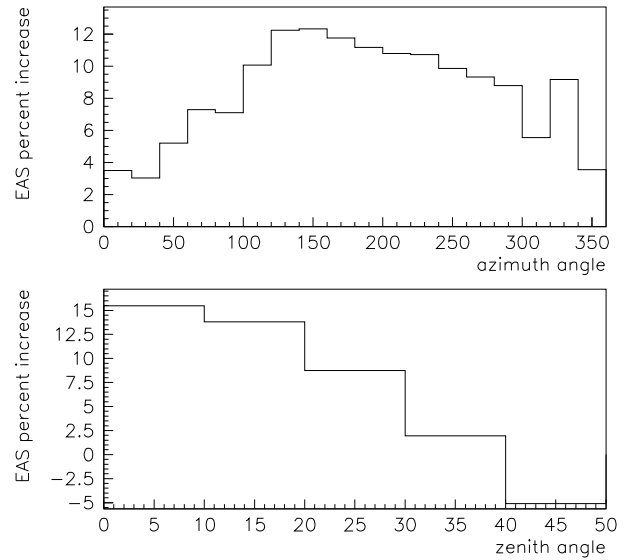
Fig. 4. Percent increase of the number of showers as a function of the azimuth and zenith angles detected during the five EAS increases added together. The azimuth angle is measured from North towards West.
