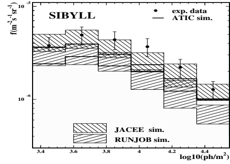
Figure 2. Measured C.I. photon density spectra (CORSIKA-SIBYLL) at distances 125 < r < 145 \text{ m} from the shower core in coincidence with \mu in MACRO. The \pm 1\sigma band expected following JACEE, RUNJOB and ATIC data is also given.
