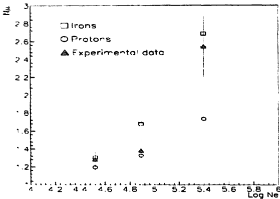
Figure 5: Correlation between N_\mu and N_e
