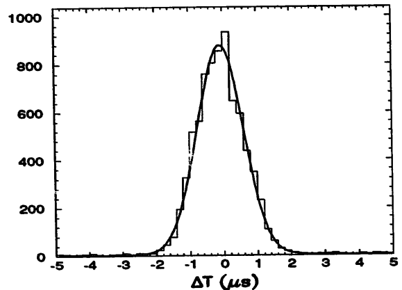
Figure 1: Time difference distribution between EAS-TOP and MACRO events.
