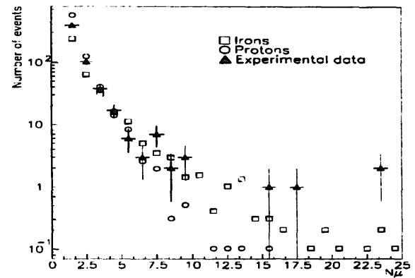
Figure 4: Muon multiplicity distributions
