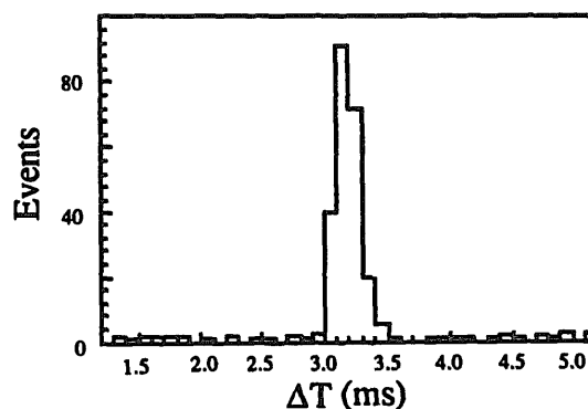
FIG. 2 Time distribution of the reconstructed events of EAS-TOP and Macro in coincidence, within 4 ms. and \Delta\psi \leq 10^\circ .
