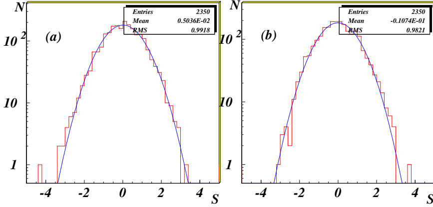
Fig. 2. Distributions of daily excesses from the Crab Nebula direction: (a) HE events, (b) LE events. The expected distributions based on Poissonian fluctuations are also shown, superimposed on the experimental ones.
