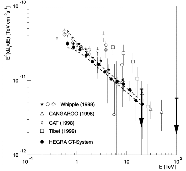
Fig. 3. Summary of VHE \gamma -ray data from the Crab Nebula (from Aharonian et al., 2000). Upper limits from the present work are indicated as large arrows.
