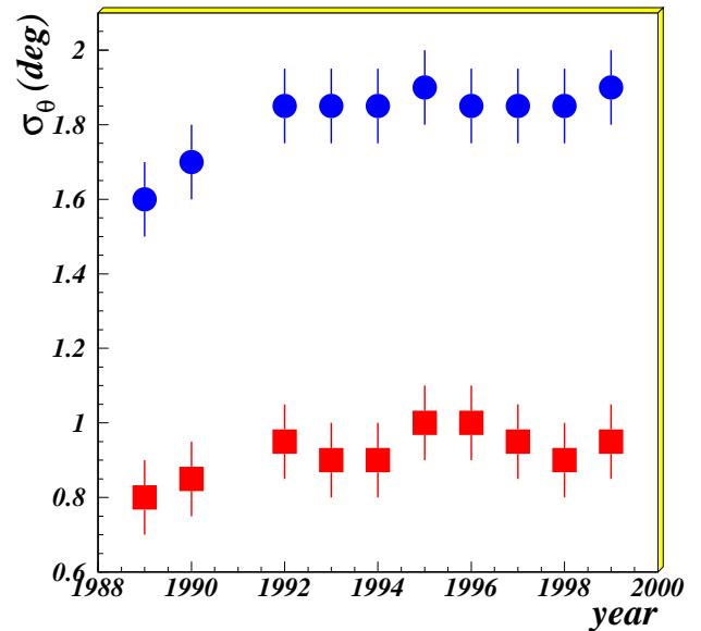
Fig. 1. Measured angular resolution vs year of operation: squares correspond to HE events, circles to LE ones.
